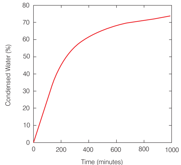
Figure 3. A typical % water recovery curve for curing a 20 ft-long hollow core Solidia Concrete slab.
